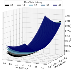
Fig. 1. Fine tuning results of micro-benchmarks
