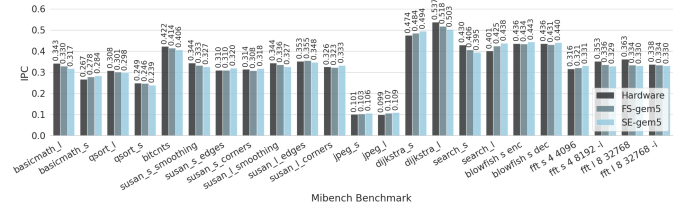
Fig. 3. Fine tuning results of the MiBench suite
