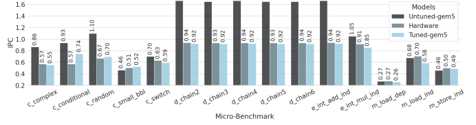
Fig. 2. Fine tuning results of micro-benchmarks
